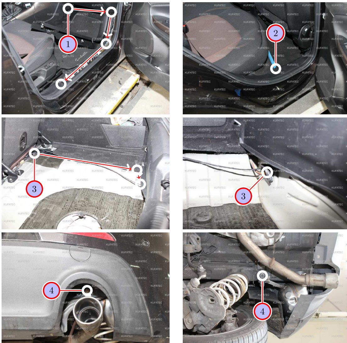
Figure 7: Cable routing / installation sound generator
