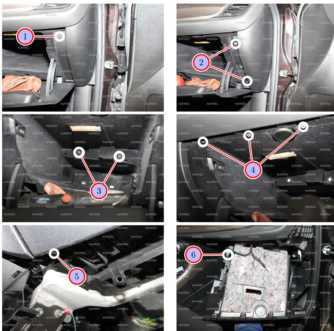
Figure 5: Removing glove compartment
