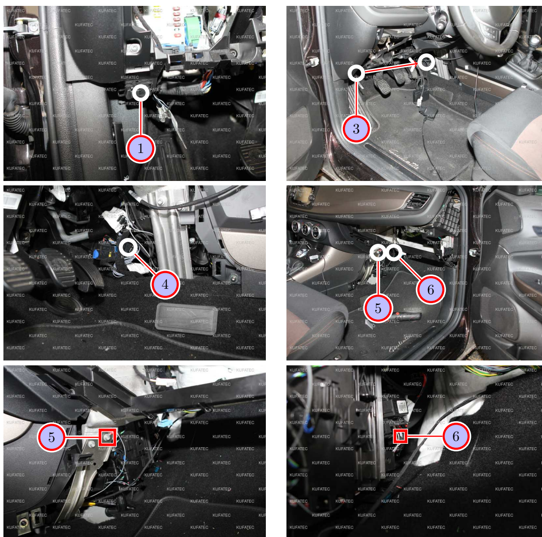
Figure 6: Connection CAN bus, ground and ignition lead
